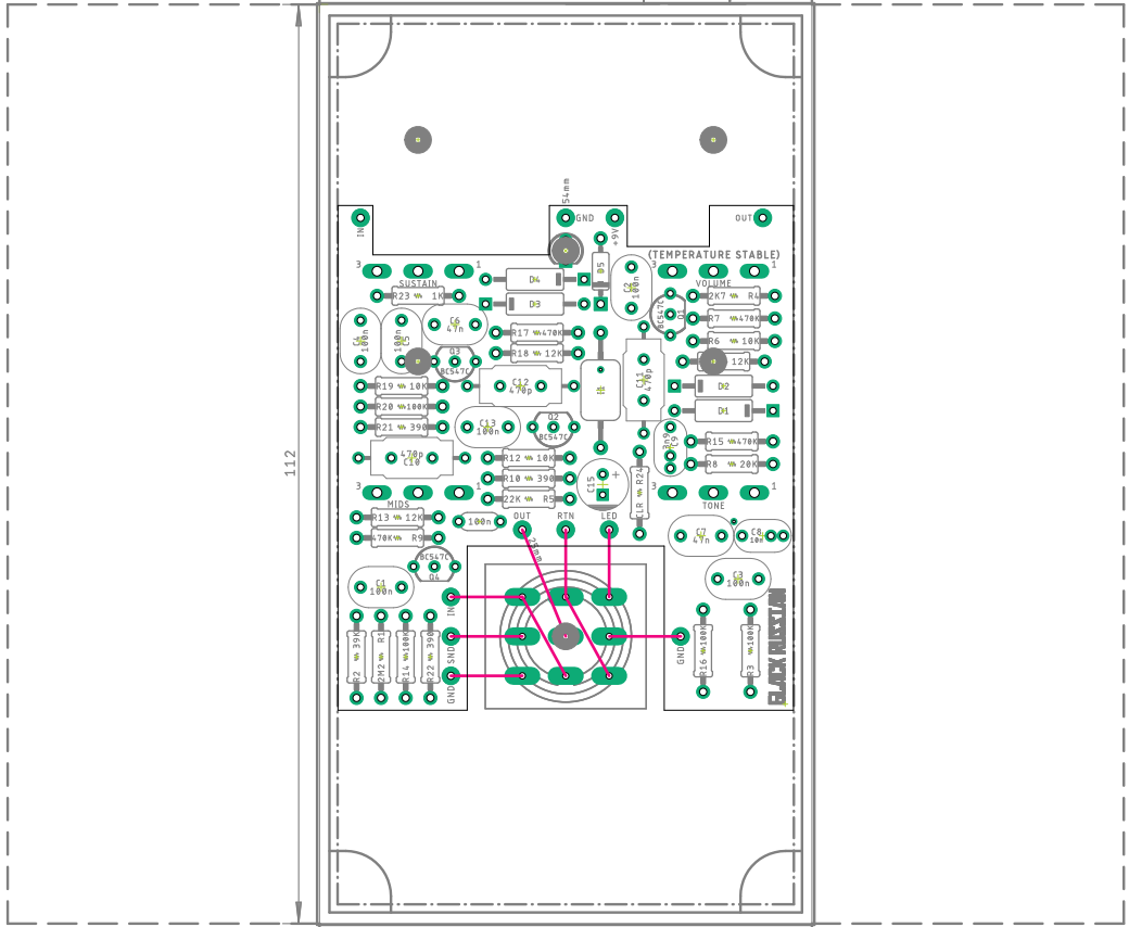
Hammond 1590BS enclosure Copyright: Darron Thornbury
